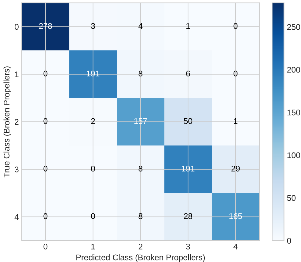
Bi-Modal AeroSync-Mamba: Test Confusion Matrix
